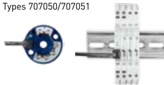
JUMO dTRANS T05 Programmable two-wire transmitter Types 707050/707051
